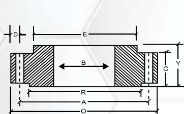
SLIP-ON FLANGE
