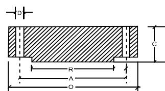
BLIND FLANGE
